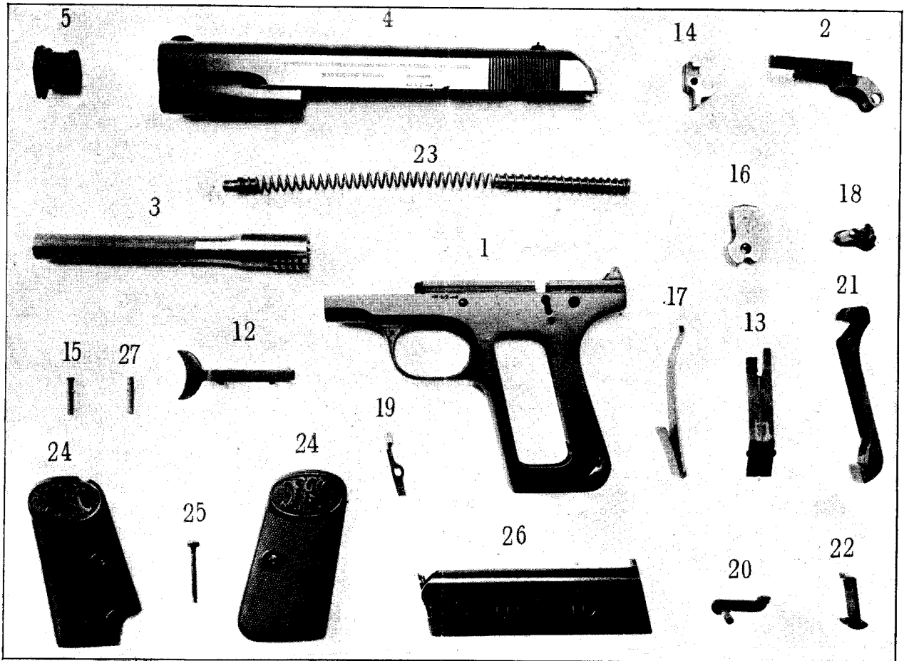
Drawing VI Parts of Pistol
